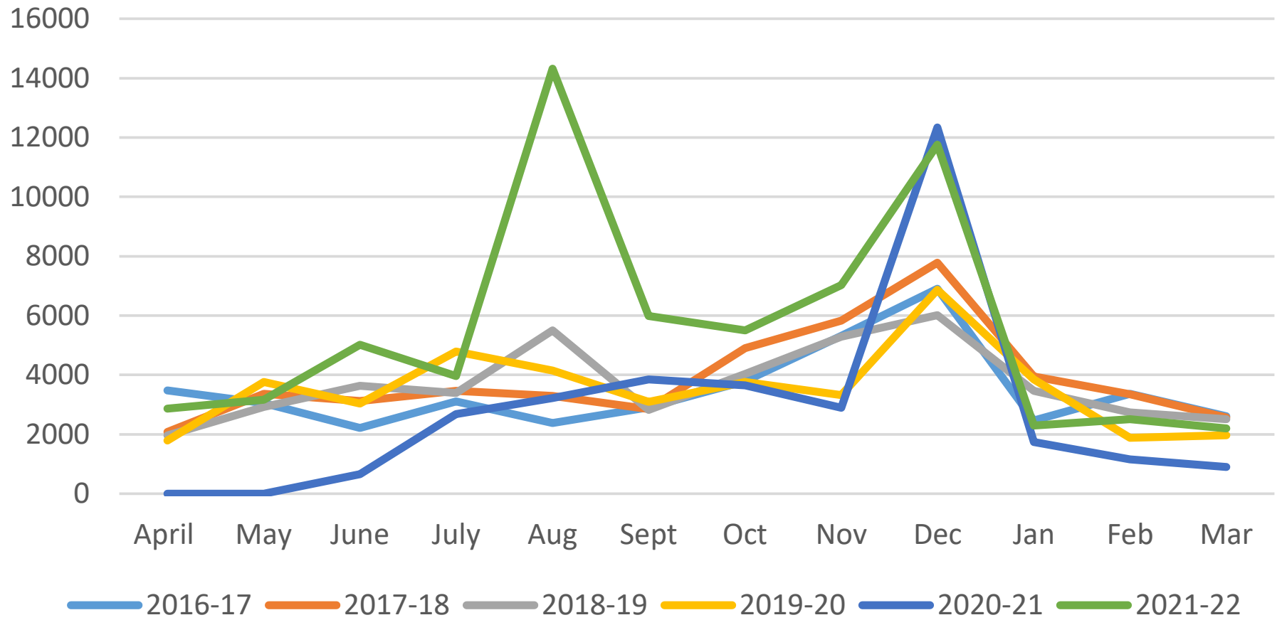
TIC income 2016-2022
